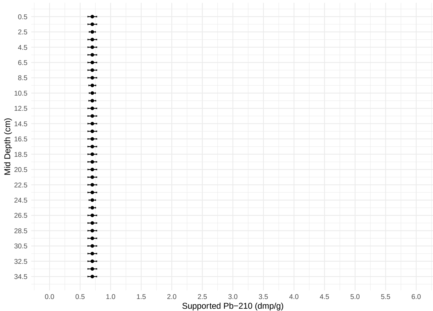
Supported Pb-210 vs Depth
